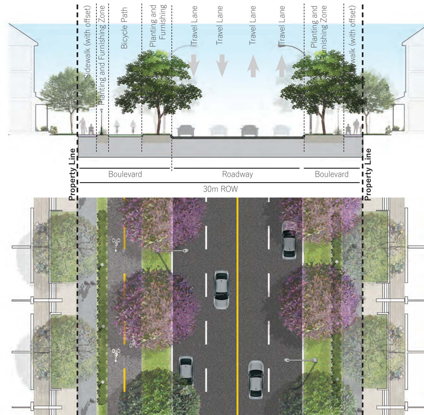
Figure 45: Type B Arterial Cross-section and Plan
