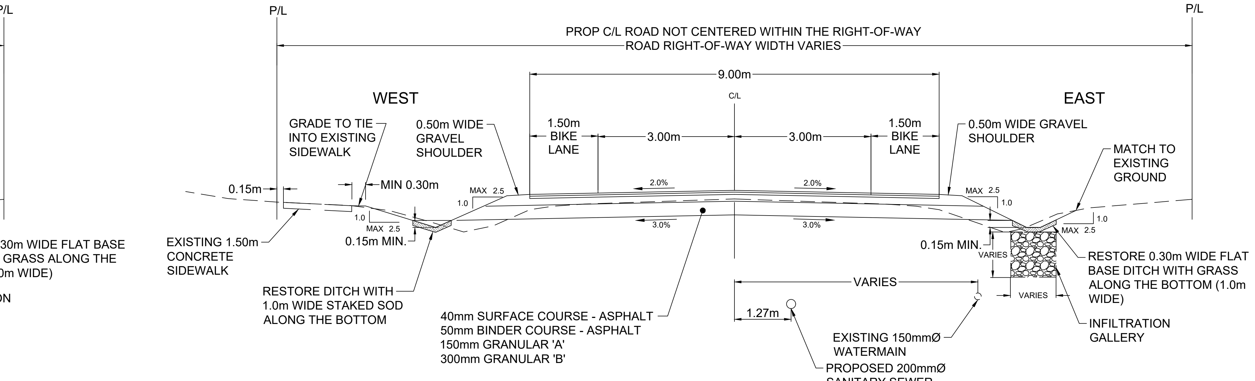
DARLINGTON BOULEVARD - TYPICAL SECTION FOXHUNT TRAIL TO HWY 2 - ST 1+550.00 TO 1+620.00
