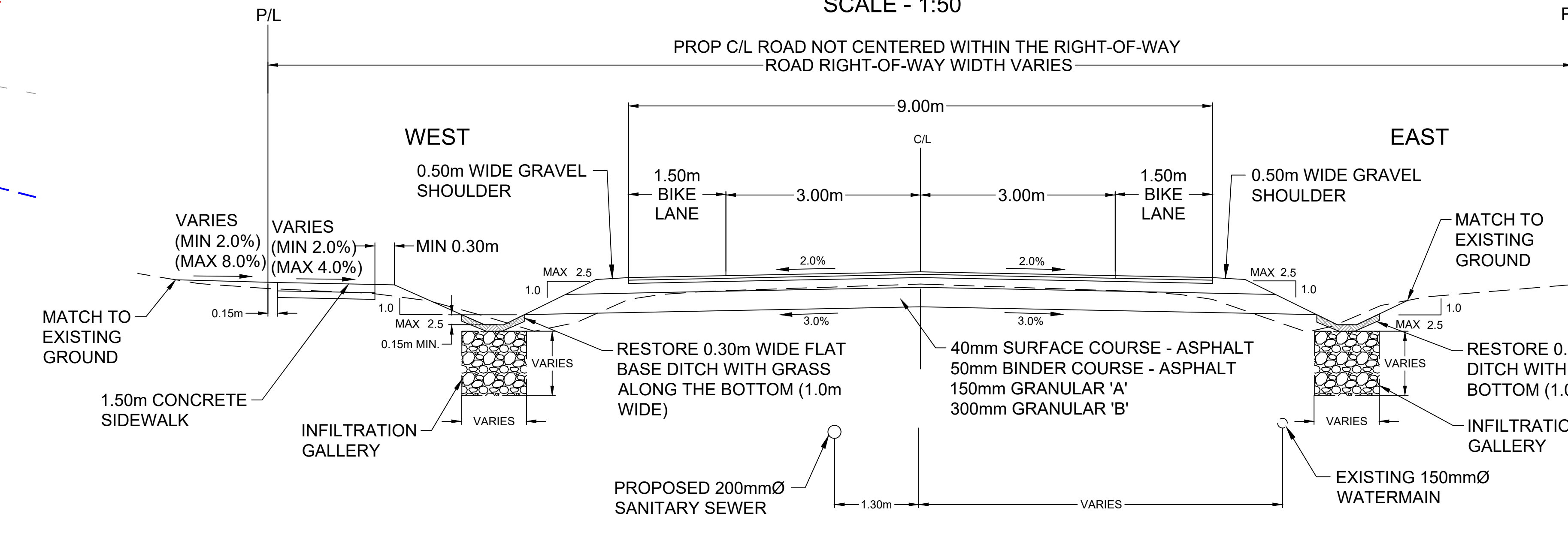
DARLINGTON BOULEVARD - TYPICAL SECTION FOXHUNT TRAIL TO HWY 2 - ST 1+000.00 TO 1+081.75
