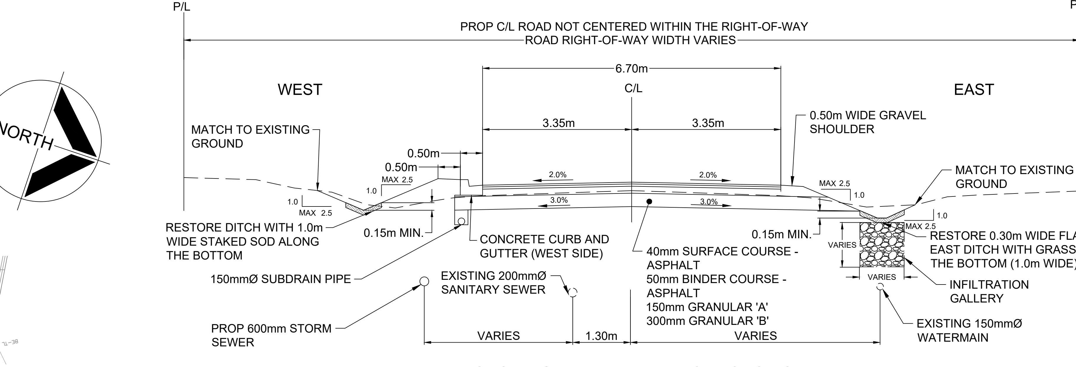
DARLINGTON BOULEVARD - TYPICAL SECTION SOUTHERN LIMIT TO FOXHUNT TRAIL - ST 0+950.00 TO 1+000.00
