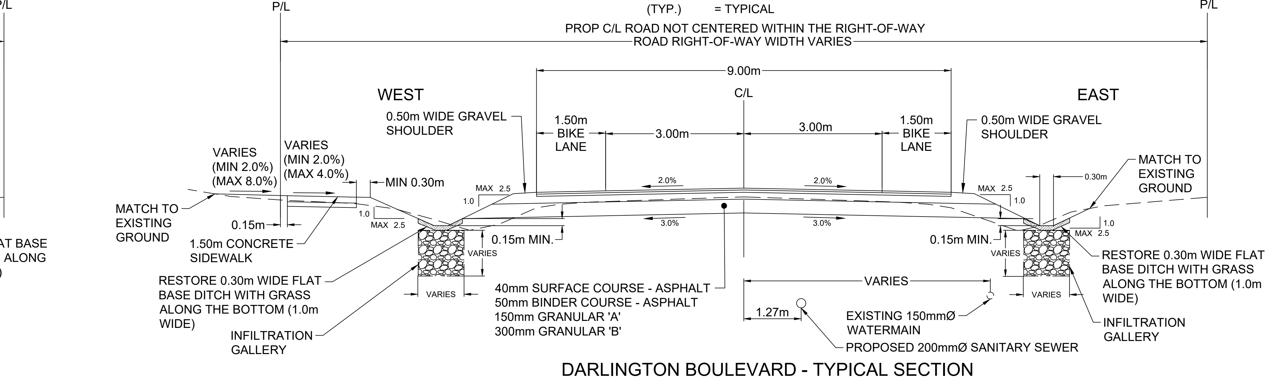
DARLINGTON BOULEVARD - TYPICAL SECTION FOXHUNT TRAIL TO HWY 2 - ST 1+081.75 TO 1+550.00
