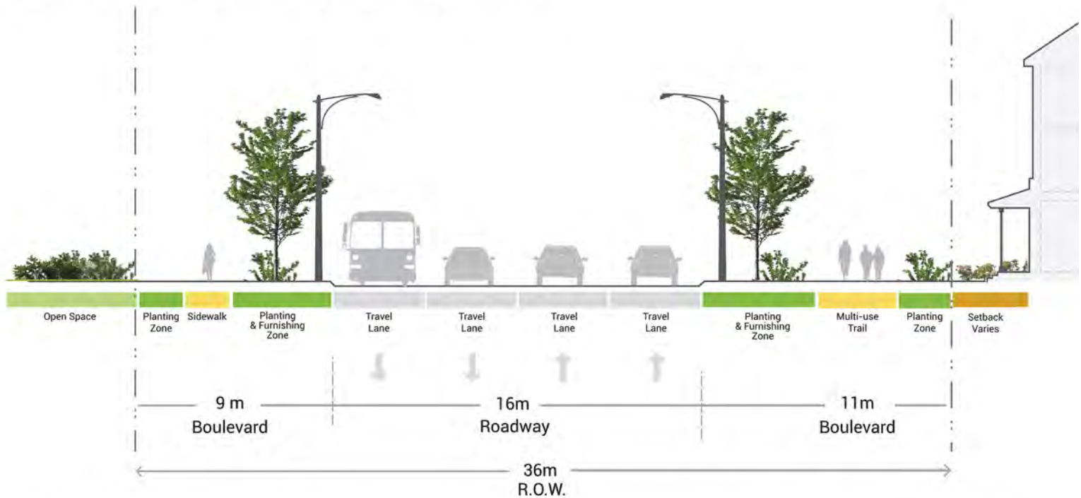
3.2 Townline Road Extension Cross-Section Option without Median (Arterial B)
