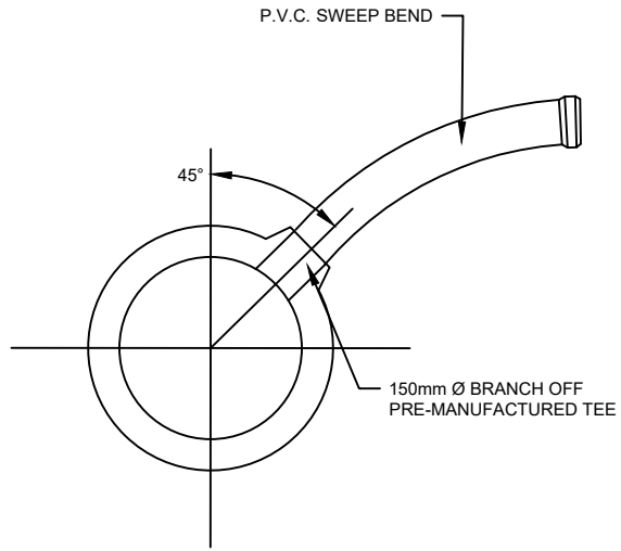
CONNECTION FOR SEWER MAINS 450mm Ø & SMALLER
