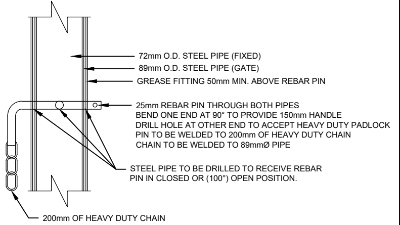
LOCKING DEVICE DETAIL
