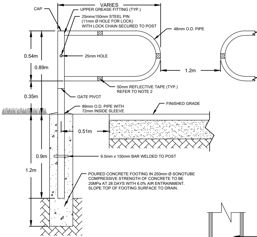
P-GATE DETAIL
